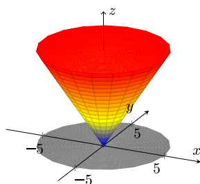
Upside-down cone of height 5 with tip at the origin. The solid is bounded by the surfaces z = \sqrt{x^2 + y^2} and z = 5 . This solid can be "projected" onto the xy -plane.
