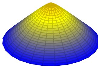
2-sheet hyperboloid
