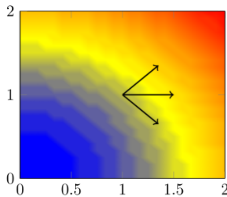
Plot where colour represents the value of \mathbf{f}(x, y) = x^2 + y^2 . The change in \mathbf{f} depends on direction
