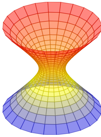
1-sheet hyperboloid
