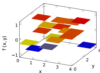
Graph of a step function
