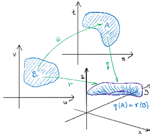
Two different representations for a given surface
