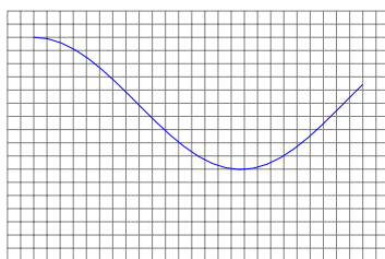
The graph of a continuous function has content zero
