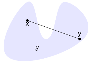
A set which is not convex.
