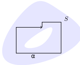
Not simply connected
