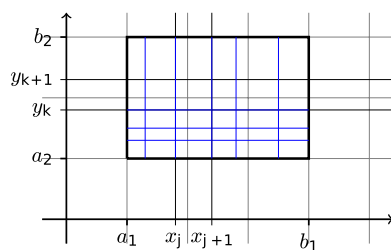
A partition of a rectangle R
