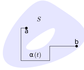
A connected set
