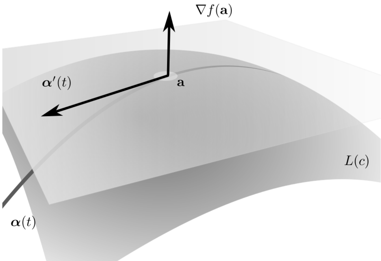
Tangent plane and normal vector
