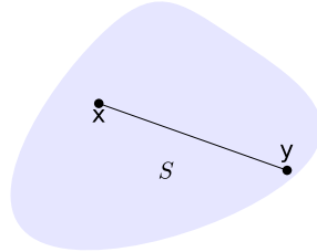
A convex set
