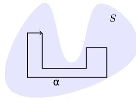
Simply connected
