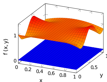
Set enclosed by xy -plane and f(x, y)
