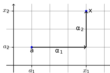
The paths \alpha_1 and \alpha_2 .
